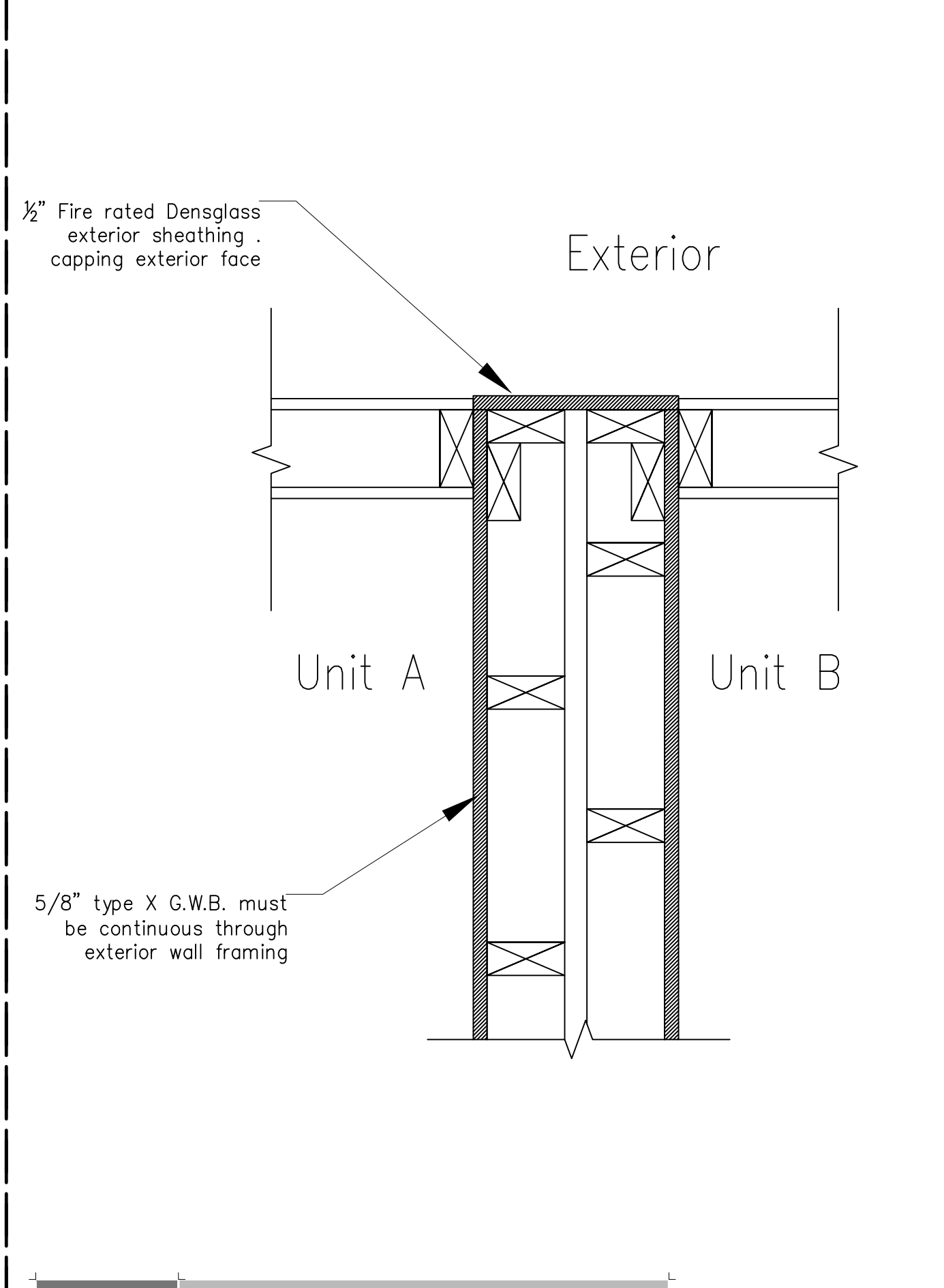
D05 Party Wall Detail - Plan SCALE 1/2" = 1'-0"
