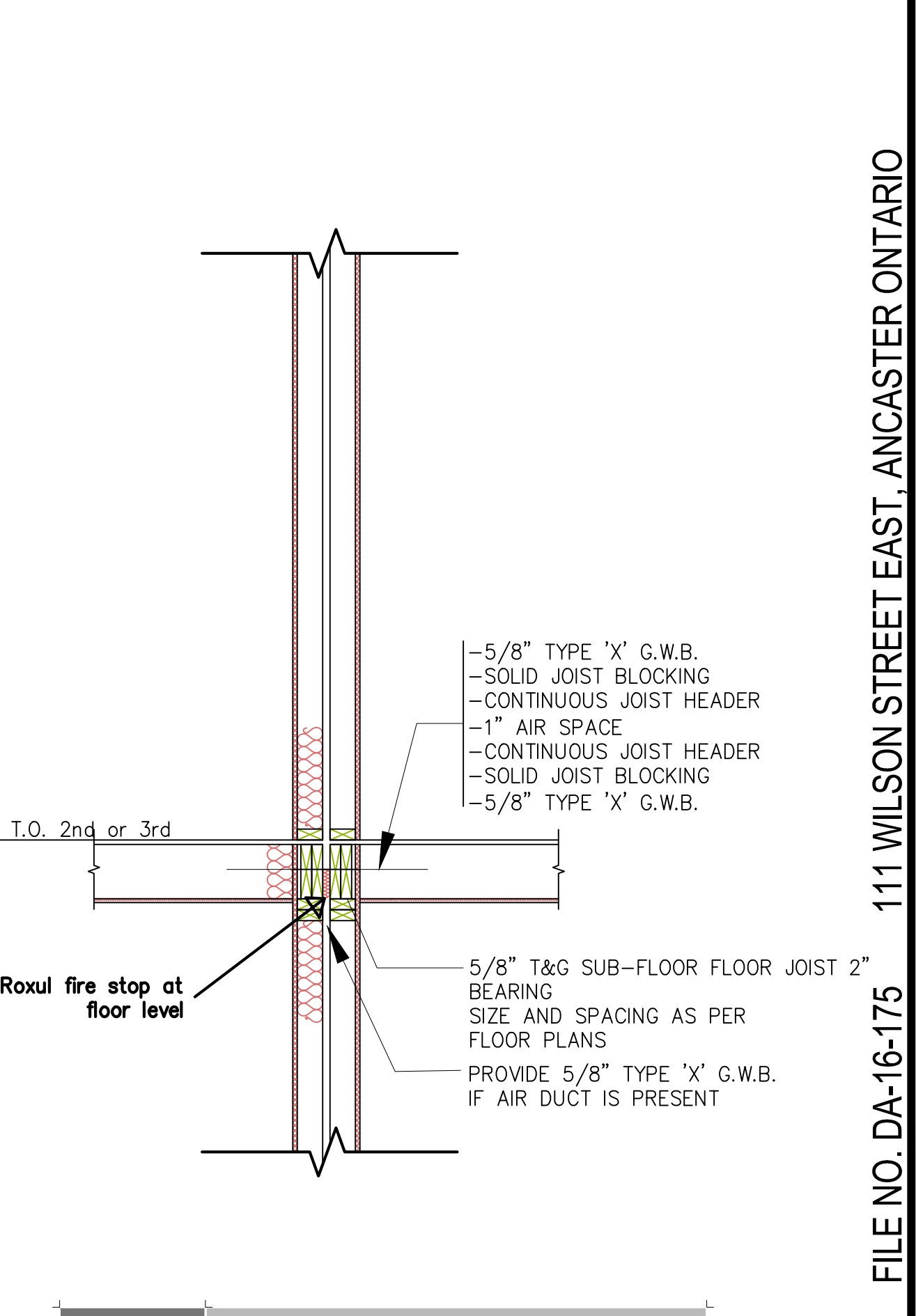
D05 Party Wall Detail SCALE 1/2" = 1'-0"
